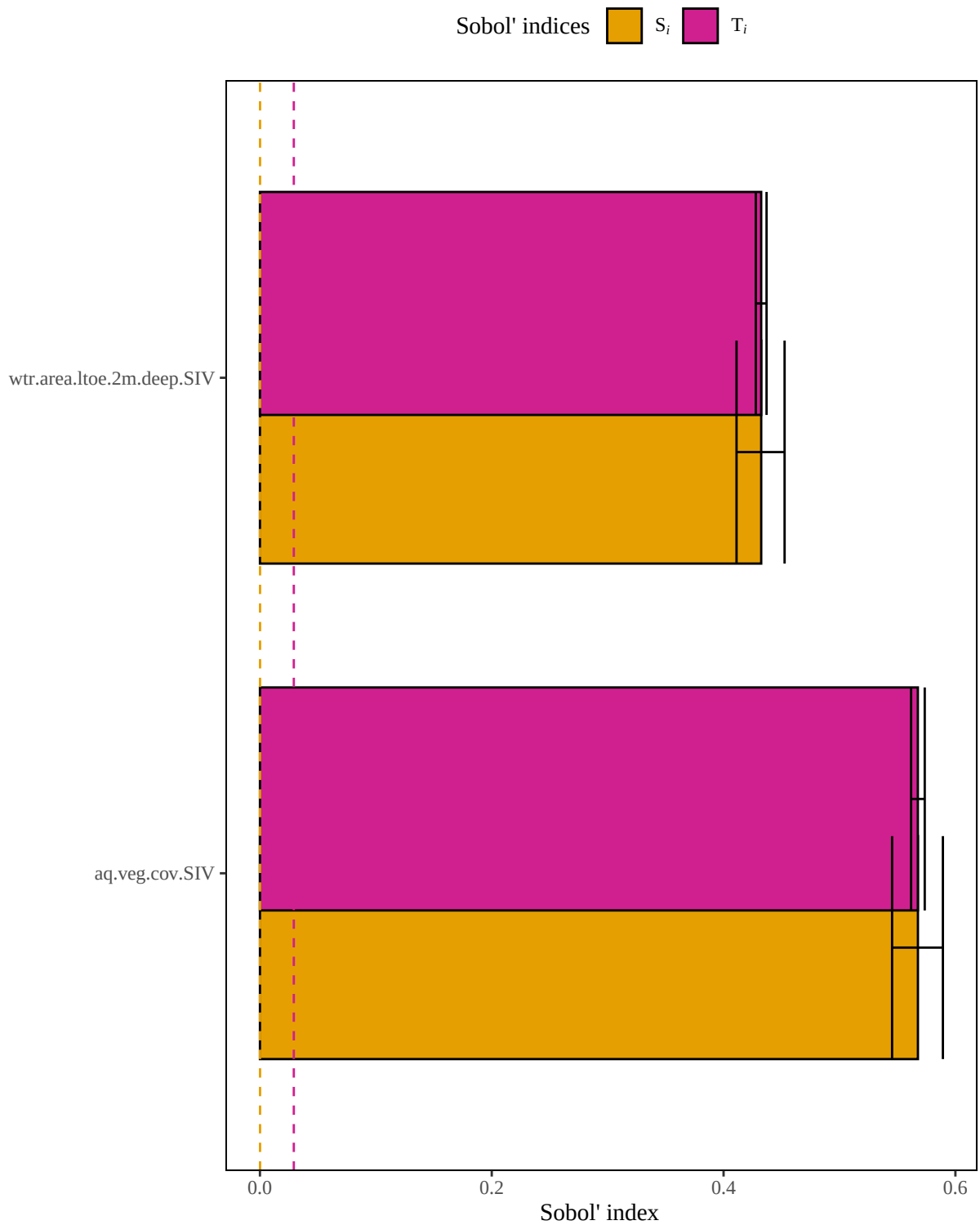
Figure 4. Results of a sensitivity analysis for the redspottednewtAquaticEntire model based on an arithmetic mean structure. Dashed lines represent baseline numerical approximation error for S_i and T_i ( i.e. , dummy variables).
